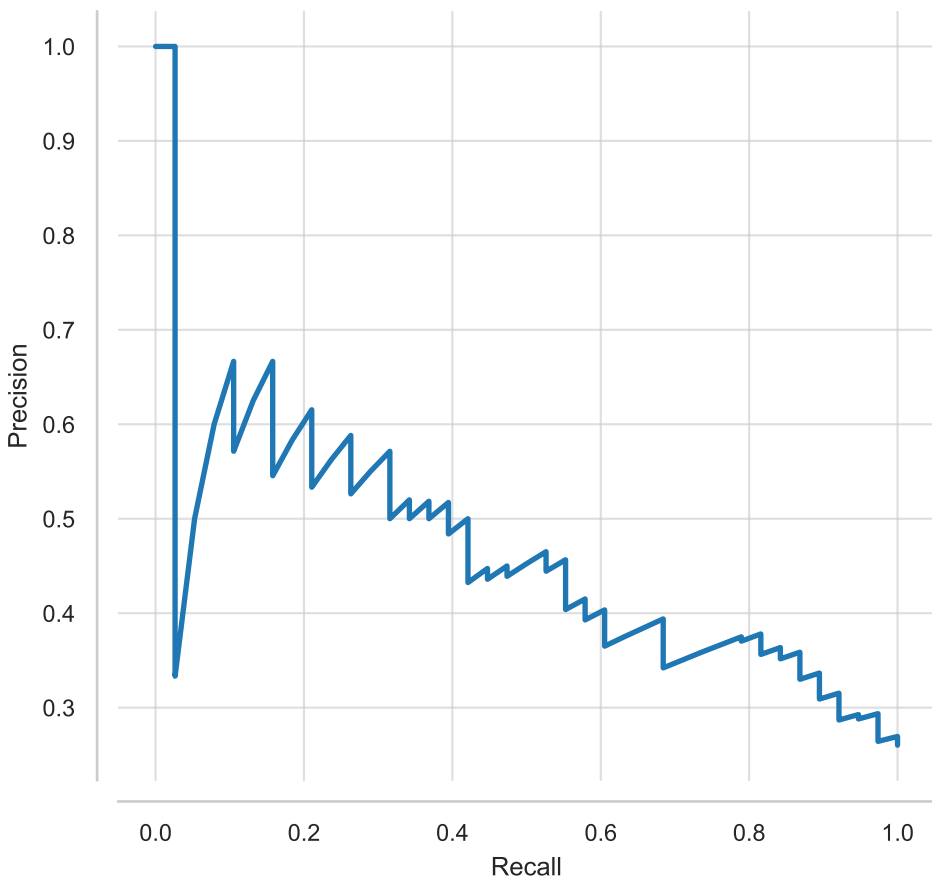
Precision-Recall Curve - LR
